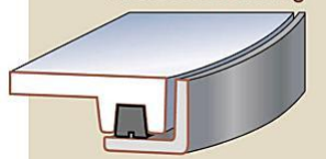
Compression Seal w/Steel Deck Ring
