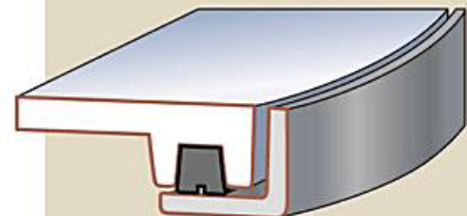
Compression Seal w/Steel Deck Ring
