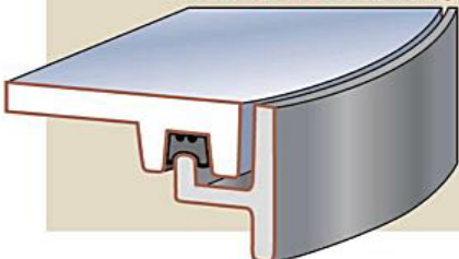
Knife Edge Seal w/Steel Deck Ring
