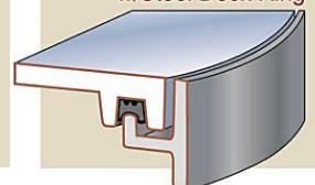
Knife Edge Seal w/Steel Deck Ring
