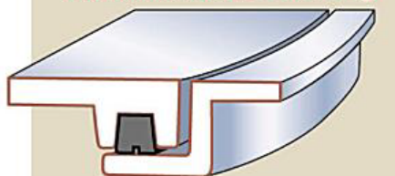
Compression Seal w/Aluminum Deck Ring
